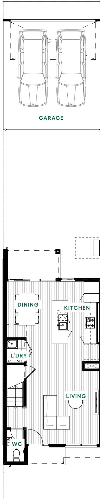
GROUND FLOOR
